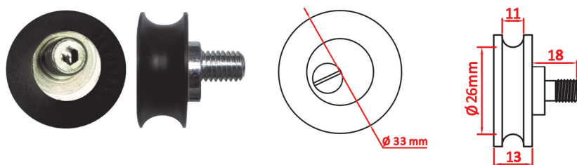
SHPE 1025 - Roldana excêntrica D 33 mm PFR-04
